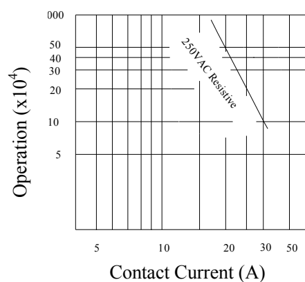
Life Curves
